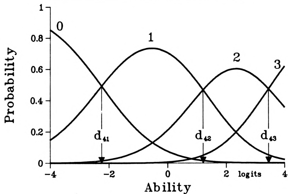
FIGURE 9.1d RESPONSE CATEGORY PROBABILITY CURVES FOR ITEM 4: COPYING SHAPES
