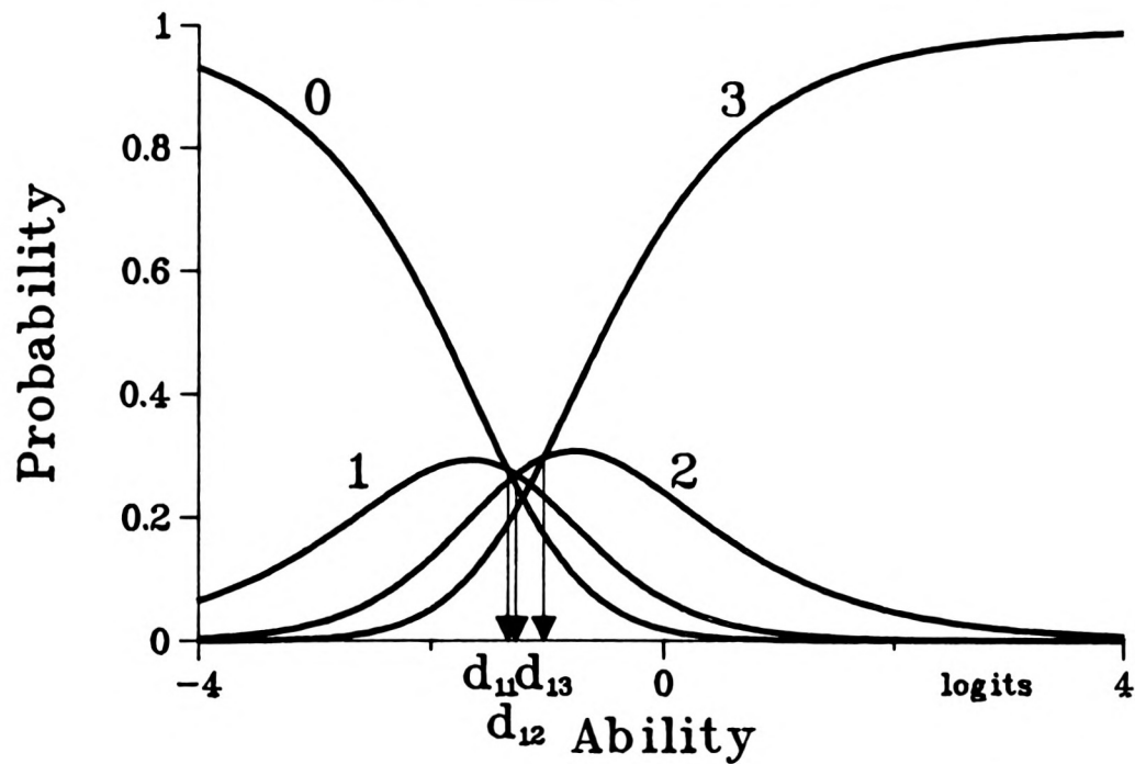
FIGURE 9.1g RESPONSE CATEGORY PROBABILITY CURVES FOR ITEM 1: MATCHING SHAPES
