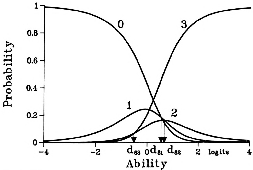
FIGURE 9.1h RESPONSE CATEGORY PROBABILITY CURVES FOR ITEM 8: SORTING BLOCKS
