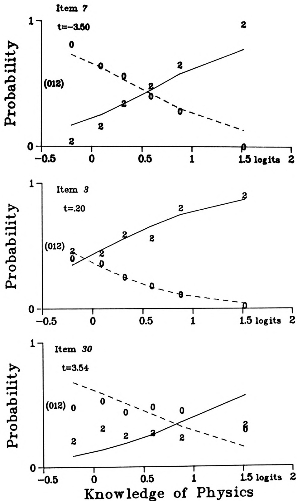
FIGURE 8.3e OBSERVED PROPORTIONS AND MODEL PROBABILITIES FOR ITEMS 7, 3 AND 30 (012) ANALYSIS
