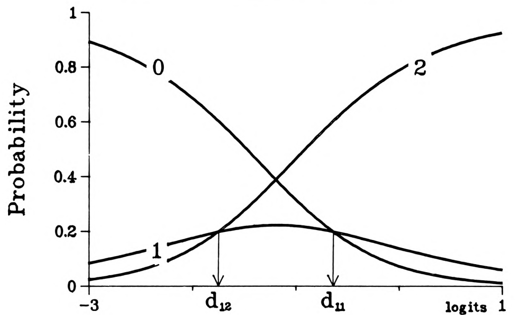
FIGURE 8.3a CATEGORY PROBABILITY CURVES FOR ITEM 1
