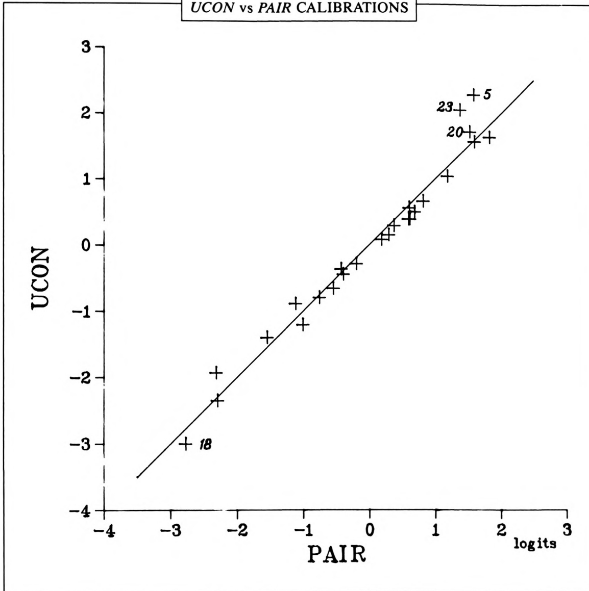
FIGURE 4.4a UCON vs PAIR CALIBRATIONS
