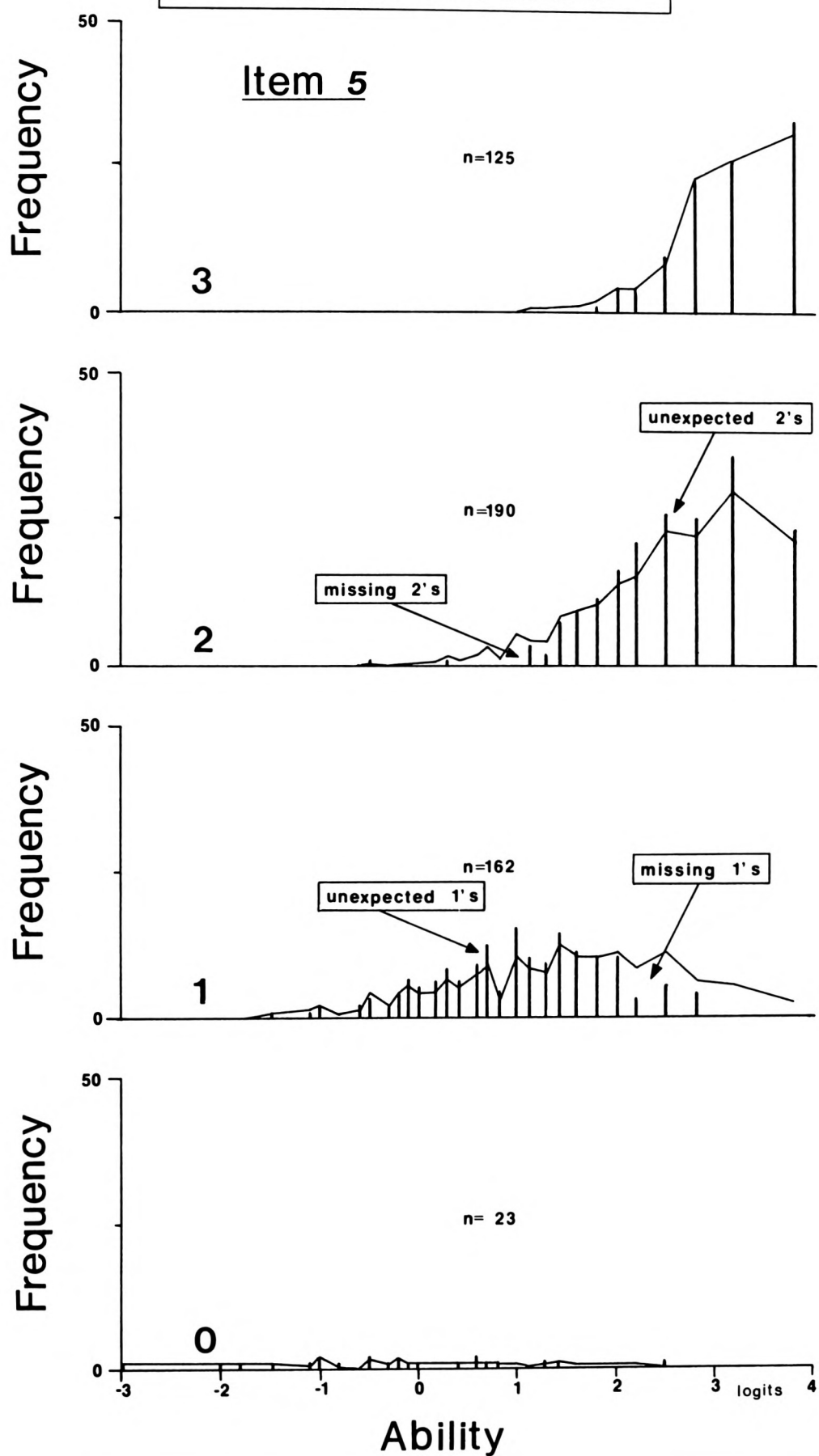
FIGURE 9.2d OBSERVED FREQUENCIES OF RESPONSE FOR ITEM 5: COPYING LETTERS
