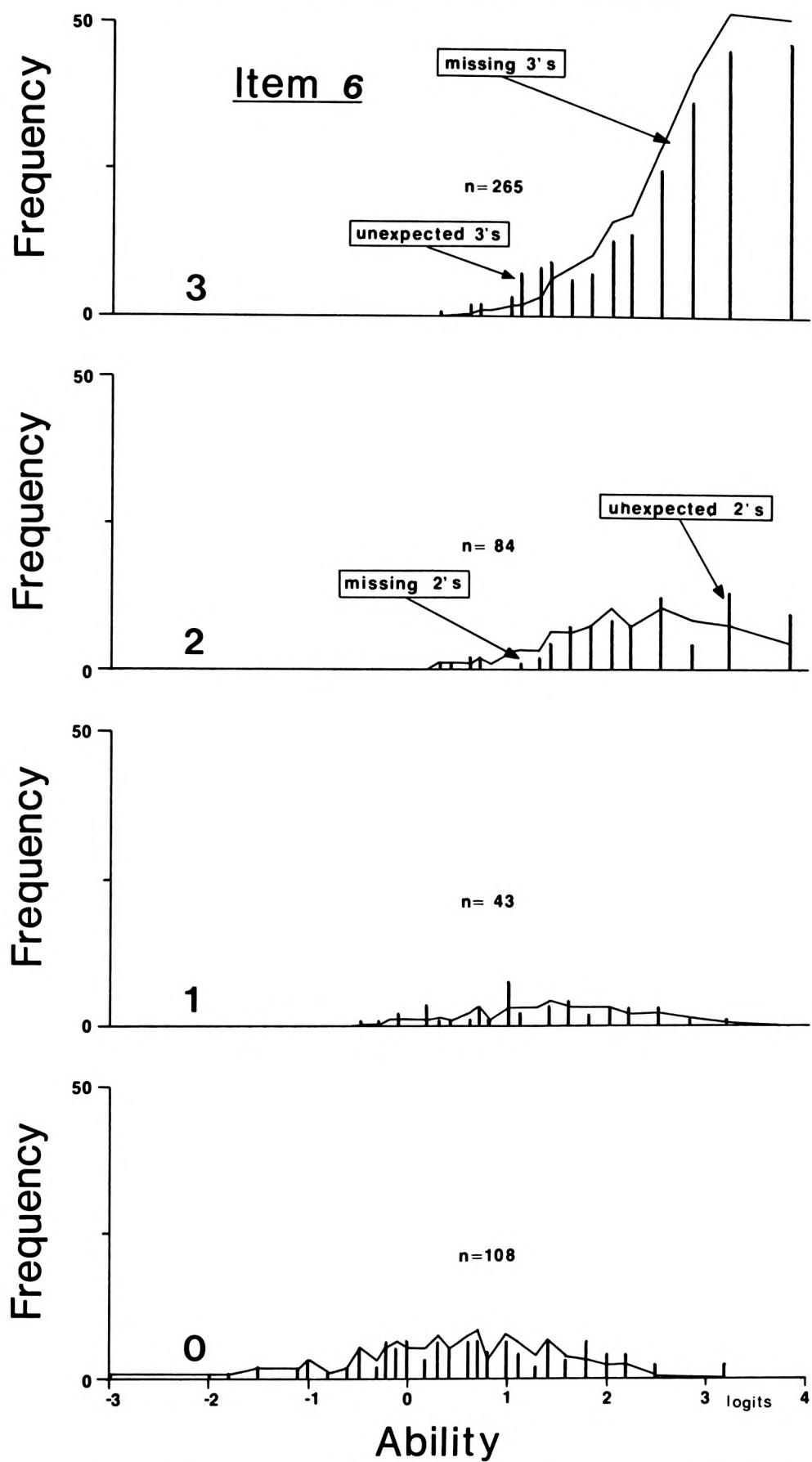
FIGURE 9.2b OBSERVED FREQUENCIES OF RESPONSE FOR ITEM 6: TOUCHING FINGERS
