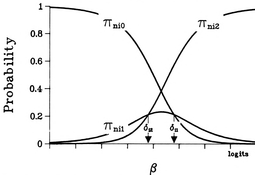
FIGURE 3.1g CATEGORY PROBABILITY CURVES FOR THE CASE \delta_{i2} < \delta_{i1}
